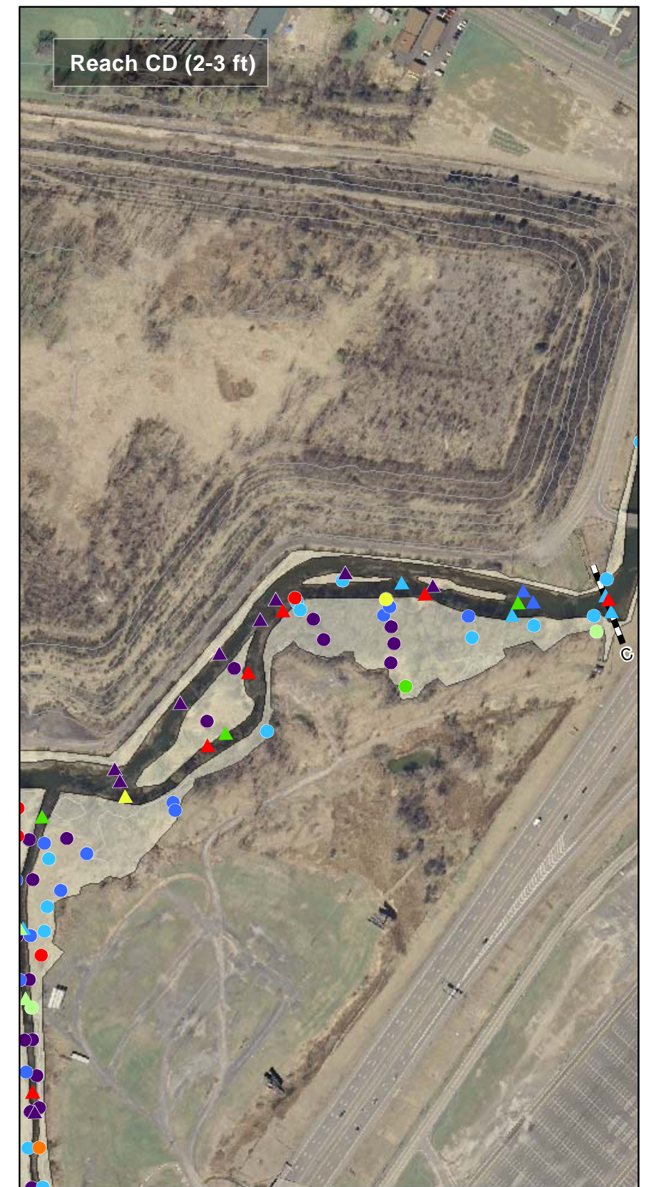
Figure 6b. Mercury Concentrations in Channel and Floodplain, Ninemile Creek Reach CD
